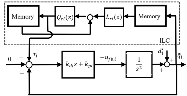
Figure 4. Command-based ILC.
