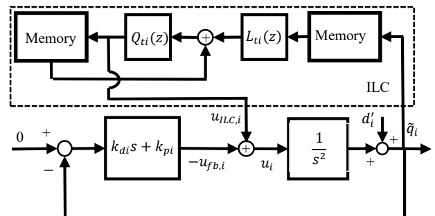
Figure 3. Control-based ILC.
