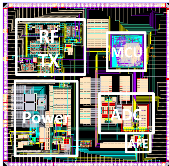
Figure 15. Layout of the proposed integrated system chip.
