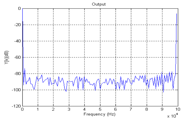
Figure 9. Simulated ADC output spectra at 200KS/s with Nyquist input.
