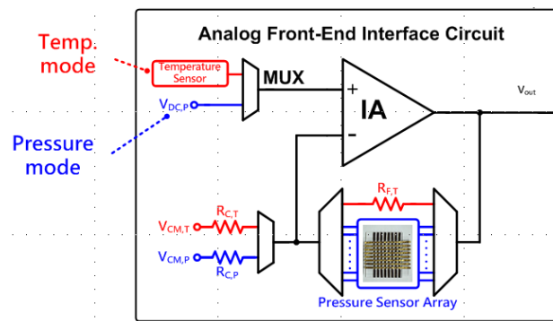
Figure 3. The schematic of analog front-end circuit.
