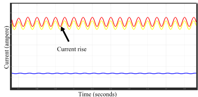
Fig. 8(b): Current waveform under RY fault
