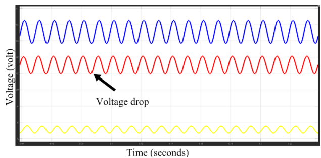
Fig. 8(a): Voltage waveform under RY fault
