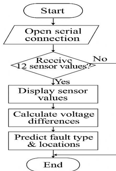
Fig. 5: Flowchart of real-time fault detection and localization process.
