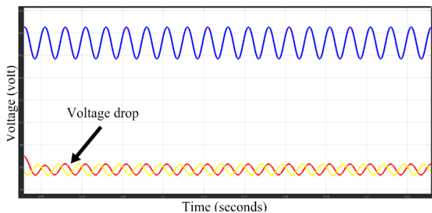
Fig. 9(a): Voltage waveform under RYG fault
