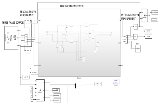
Fig. 1: Complete MATLAB Simulink Model of Underground Power Cable
