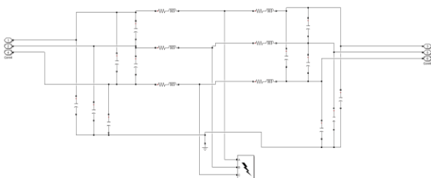
Fig.2: Simulink Subsystem Model of Underground Power Cable
