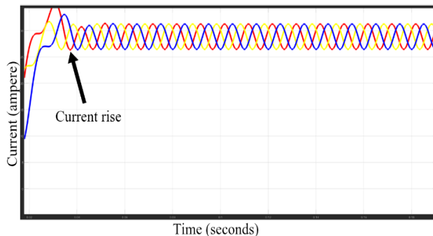
Fig. 10(b): Current waveform under RYBG fault
