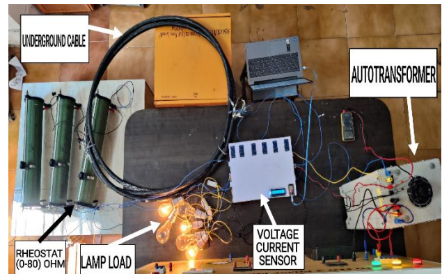
Fig.3 : Experimental Hardware Setup under Operating Condition
