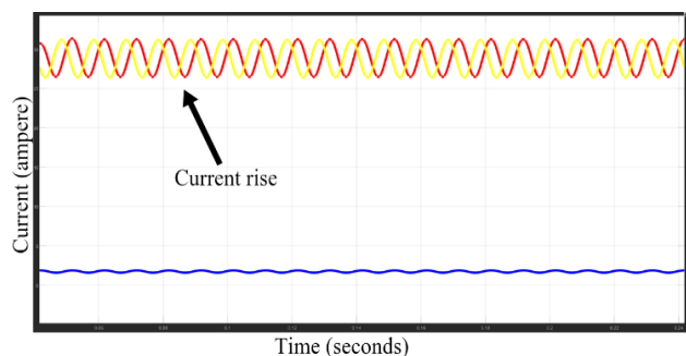
Fig. 9(b): Current waveform under RYG fault
