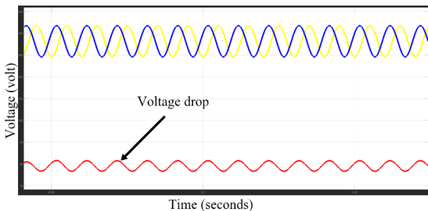
Fig. 7(a): Voltage waveform under RG fault
