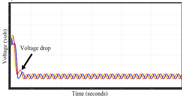
Fig. 10(a): Voltage waveform under RYBG fault
