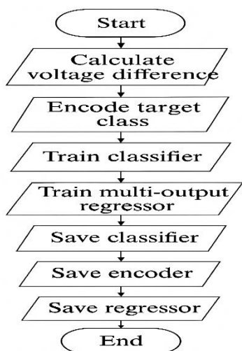
Fig. 4: Flowchart of the machine learning model training
