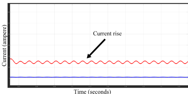
Fig. 7(b): Current waveform under RG fault
