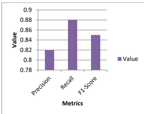
Figure 5. Precision, Recall, and F1-Score Comparison
