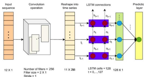
Figure 2(b). Architecture of the Proposed LSTM-Based Hypoglycemia Forecasting Model
