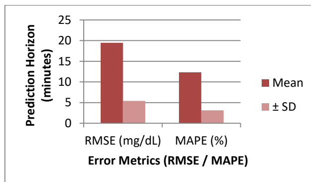
Figure 6. Prediction Error with Uncertainty (Mean ± SD)
