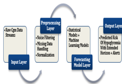
Figure 1(b). Forecasting Framework for Nocturnal Hypoglycemia
