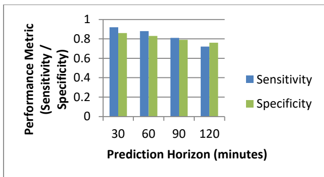
Figure 4. Sensitivity and Specificity at Different Prediction Horizons
